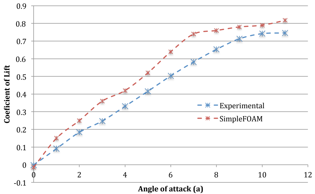
Figure 22: Comparison of Coefficients of Lift at U = 12.55 m/s
