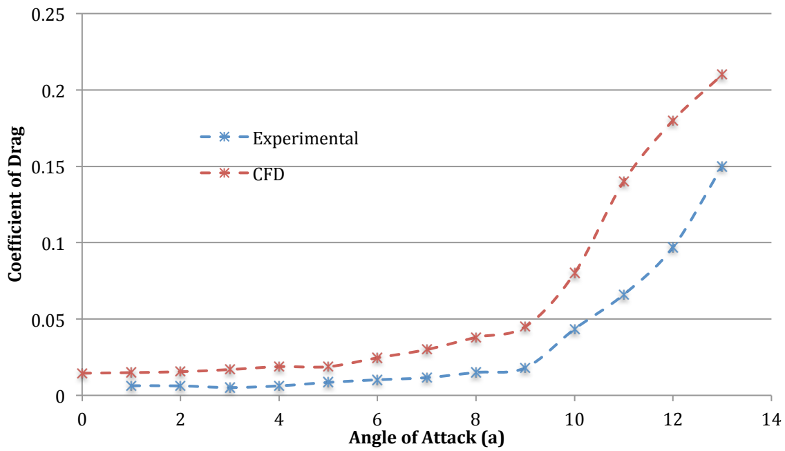
Figure 17: Comparison of Coefficients of Drag at U = 9.45 \text{ m/s}
