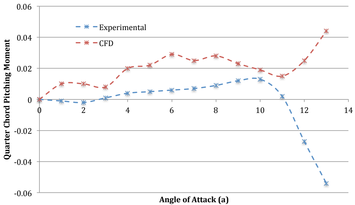
Figure 18: Comparison of Quarter Chord Pitching Moments at U = 9.45 \text{ m/s}
