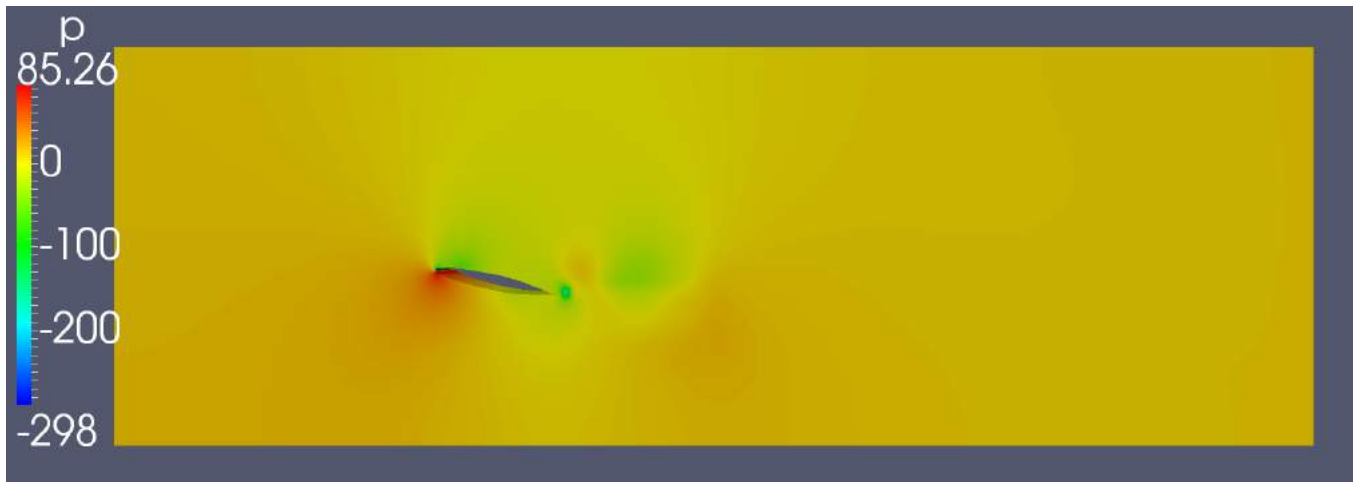
Figure 21: Pressure Field of NACA66-012 Foil at U = 12.55 m/s and \alpha = 11^\circ
